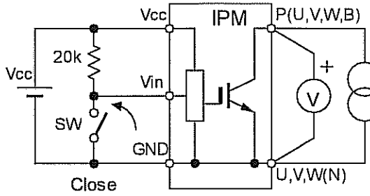
Figure4. Vce(sat) Test Circuit (Terminal)
