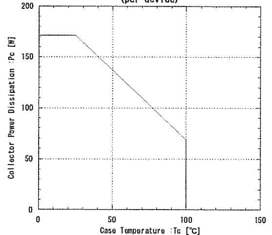
Power derating for IGBT (max.) (per device)
