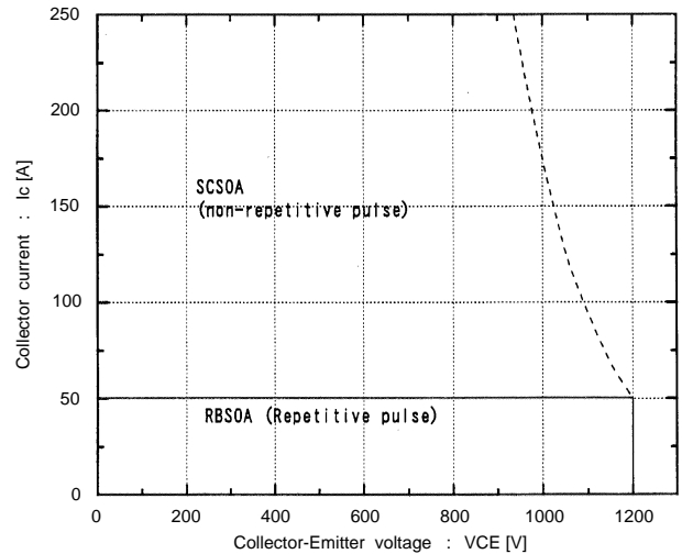
Reversed biased safe operating area +VGE=15V, -VGE ≤ 15V, Tj ≤ 125°C, RG ≥ 51 ohm
