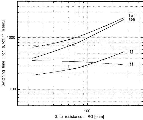
Switching time vs. RG Vcc=600V, Ic=25A, VGE=±15V, Tj=25°C
