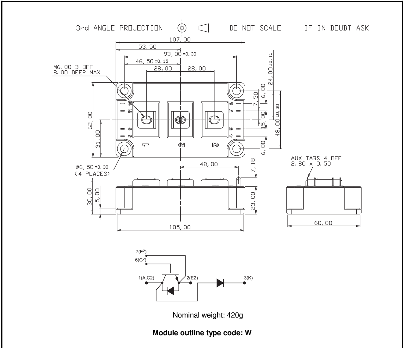
Fig.11 Package details
