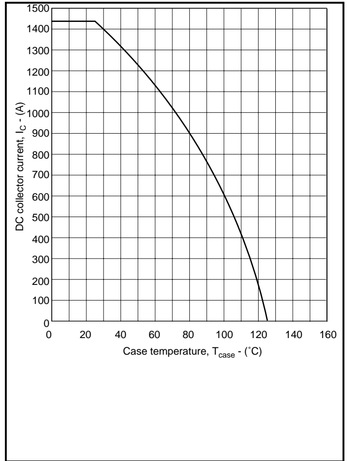
Fig. 15 DC current rating vs case temperature
