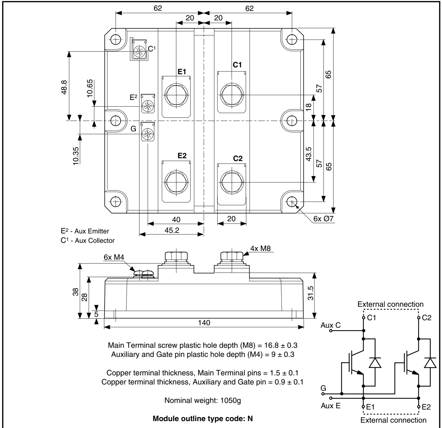
Fig. 11 Package details
