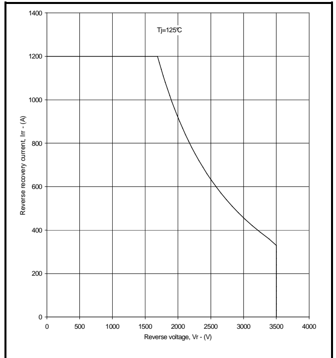
Diode reverse bias safe operating area
