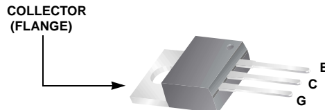
JEDEC TO-220AB (ALTERNATE VERSION)
